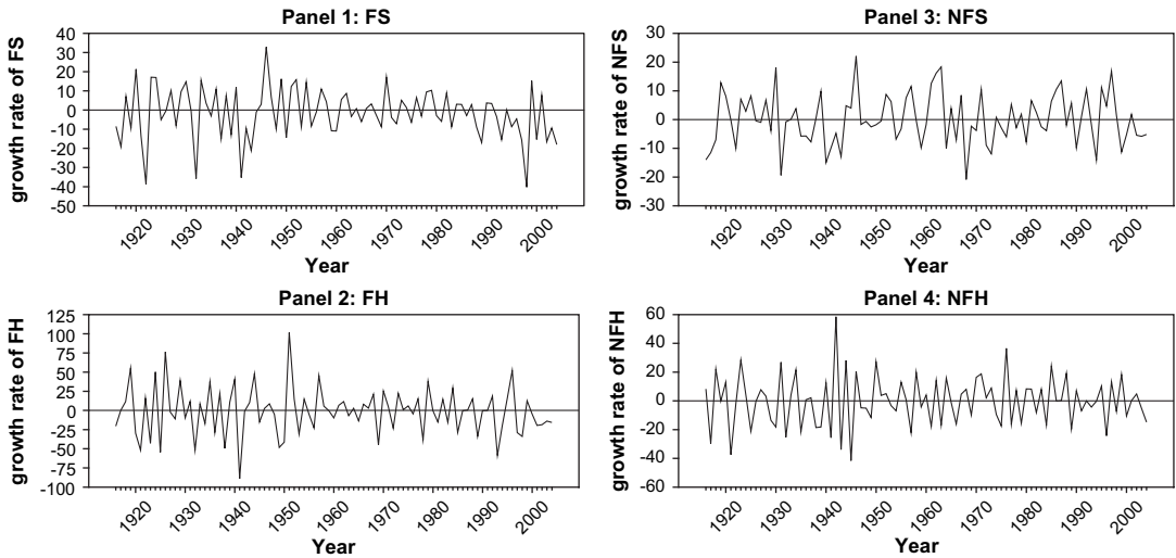
FIGURE 2 Plots of the Series Growth Rates
